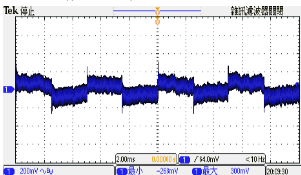
Figure 7 : Transient Response at Output step load ( V_{in} : Typical, 25~50% of output current; \Delta I_o/\Delta t = 1\text{A}/\mu\text{s} )
